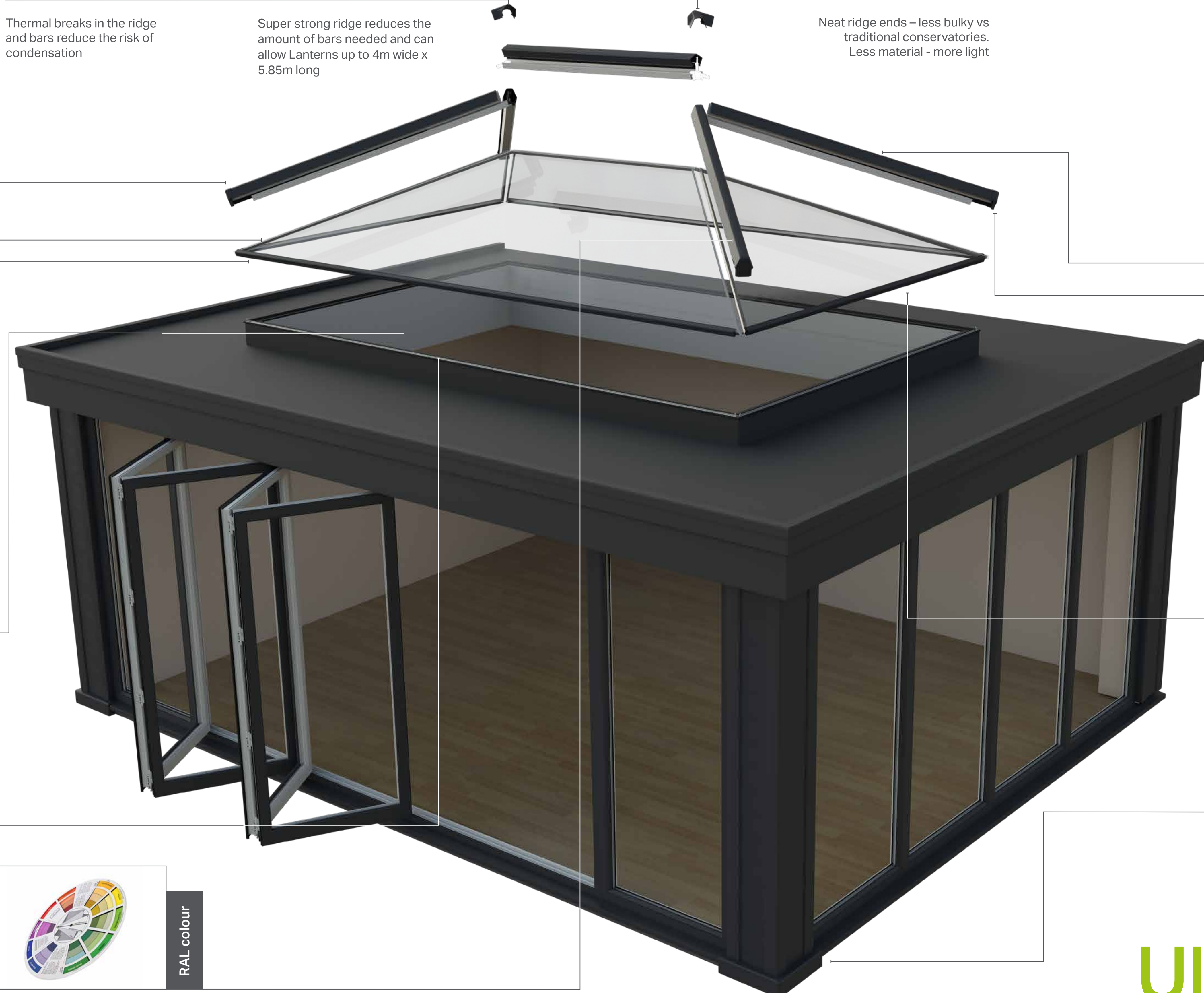
Thermally broken
